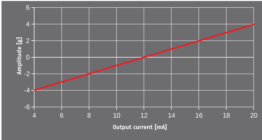
Figure 1: Output current
